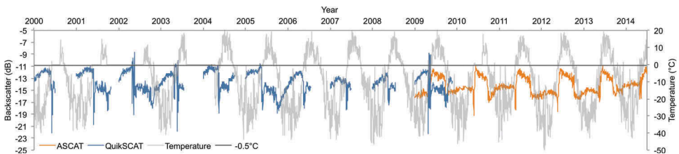
Figure 2. Example time series of scatterometer backscatter and in situ air temperature ( T_{\text{met}} ) at Koluktak, 2000–2014 (shown in Figure 1). Daily vertically-polarized (V-pol) time series of QuikSCAT (blue) and ASCAT (orange) backscatter are plotted with in situ air temperature (light gray). The horizontal gray line marks -0.5^{\circ}\text{C} , the threshold used in the melt proxy.
