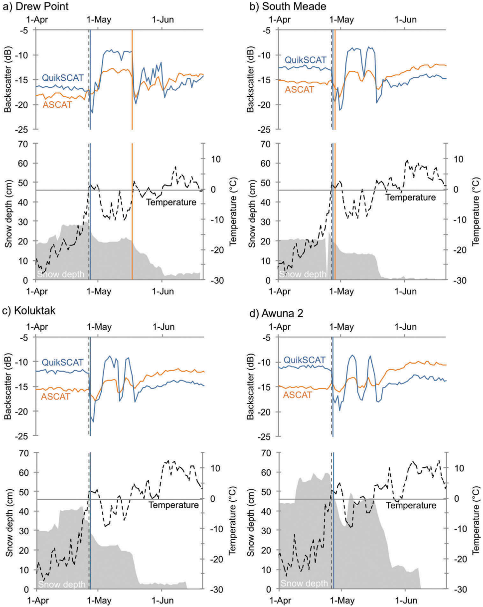
Figure 3. Time series of scatterometer and in situ data at meteorological station sites during the 2009 melt season (1 April – 20 June). Sites are ordered by distance from coast (refer to Figure 1): a) Drew Point, b) South Meade, c) Koluktak, and d) Awuna 2. Daily time series of vertically polarized sent and received (V-pol) QuikSCAT (blue line) and ASCAT (orange line) are plotted above in situ snow depth (solid gray) and air temperature ( T_{\text{met}} ) (dashed black line). Vertical lines indicate melt onset dates detected by QuikSCAT (blue), ASCAT (orange), and T_{\text{met}} (dashed).
