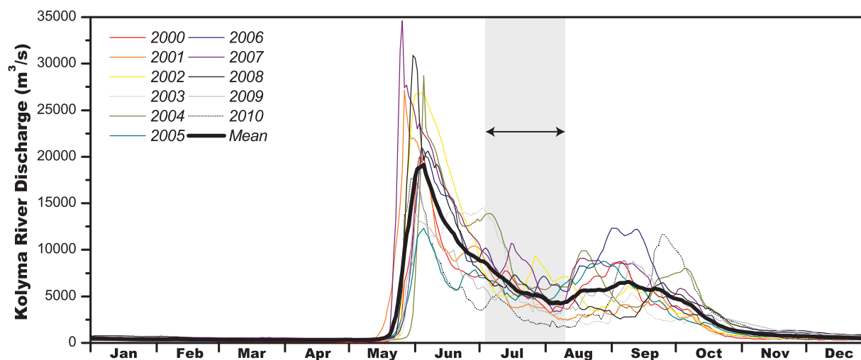
Figure 2. Daily discharge of the Kolyma River (adjusted to Cherskiy, Russia, 160 km downstream of the gauging station) for the years 2000–2010 (color coded lines) and mean discharge (black line). The Kolyma is characterized by peak flow in early June, followed by summer base flow. There is often a less pronounced peak in discharge late in the summer, usually during late August or September. The grayed out area of the hydrographs indicates the timeframe examined in this study (6 July through 10 August).
