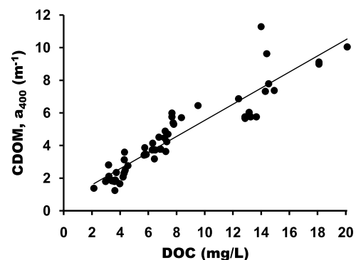
Figure 3. The relationship between dissolved organic carbon (DOC) and CDOM in the Kolyma River, using 54 field observations from July 2008 and 2009. ( CDOM = 0.494(DOC) + 0.605 ; R^2 = 0.86 ; p value < 0.01 ; equation (3)).
