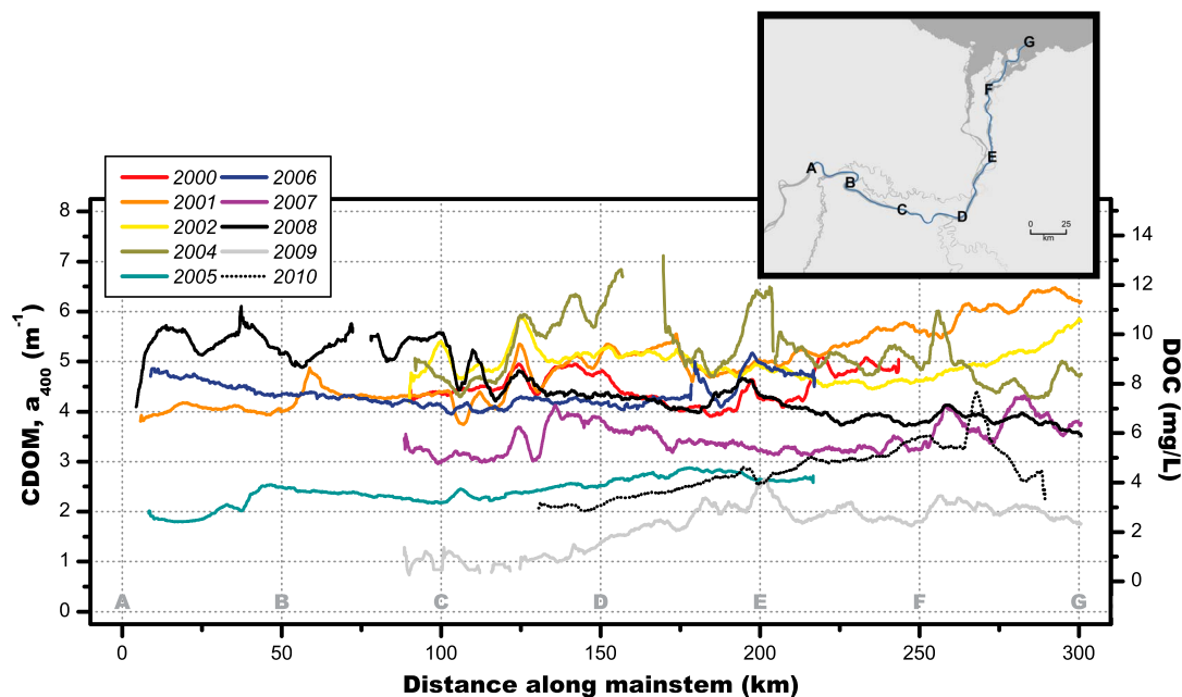
Figure 6. Profiles of CDOM and DOC extracted from satellite-based mapped concentrations.
