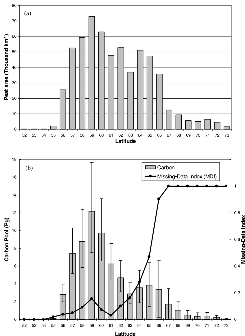
Figure 8. Latitudinal distribution of (a) peatland area, and (b) carbon pool. A bimodal distribution in both histograms indicates that the carbon pool is split E-W at \sim 63^\circ\text{N} by the Sibirske Uvaly Hills. The southern pool contains about 395,000 km 2 of peatlands and comprises \sim 76\% of the carbon pool. Though the northern peatlands occupy 33% of the total peatland area, they comprise only \sim 24\% of the carbon pool. Error bars on Figure 8b represent carbon pool uncertainties for each 1-degree latitude (Section 6.2). Also shown is the missing-data index (MDI) as a function of the latitude. The MDI increases sharply northward of 63^\circ\text{N} owing to a paucity of field data. However, this problem is mitigated by reduced peatland area and thickness, resulting in substantially less carbon storage at high latitudes.
