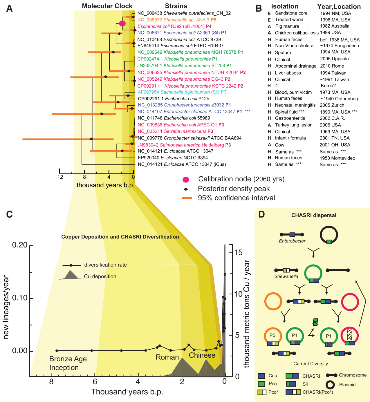
Fig. 7. —Origin and diversification of CHASRIs. (A) Chronogram generated in BEAST version 1.7.1 (Drummond and Rambaut 2007) from a CHASRI multigene nucleotide alignment. The aligned region includes silE , cusSRCFBA , and DUF411 . Support values are out of 100 ML bootstraps. Taxon name coloring corresponds to plasmid synteny according to Mauve alignment (supplementary fig. S3, Supplementary Material online). Scale is calibrated with a 2,060-year minimum divergence between subterranean CHASRI and the most closely related surface CHASRI. (B) Description of CHASRI-containing strains in (A). Bold “E,” “A,” and “H” denote isolation in environment, agriculture, and hospital, respectively. Additional metal resistances are as reported in genome publications (parentheses indicate minimum resistance where complete genome was not available at the time of analyses). (C) Graph of estimated global copper deposition due to human activity, reproduced from Hong et al. (1996). (D) Reconstruction of dispersal of CHASRIs, based on branching order in figure 5 and (A), and plasmid distributions shown in (A). A parsimonious reconstruction suggests that a chromosomal cus became linked with a plasmid pco in Enterobacter , and the resultant cluster was then distributed to new plasmids following insertion into chromosomes. Integration into a Shewanella chromosome resulted in recombination of CHASRI cus with native Shewanella pco , and sil clusters resulted from loss of pco from CHASRI.
