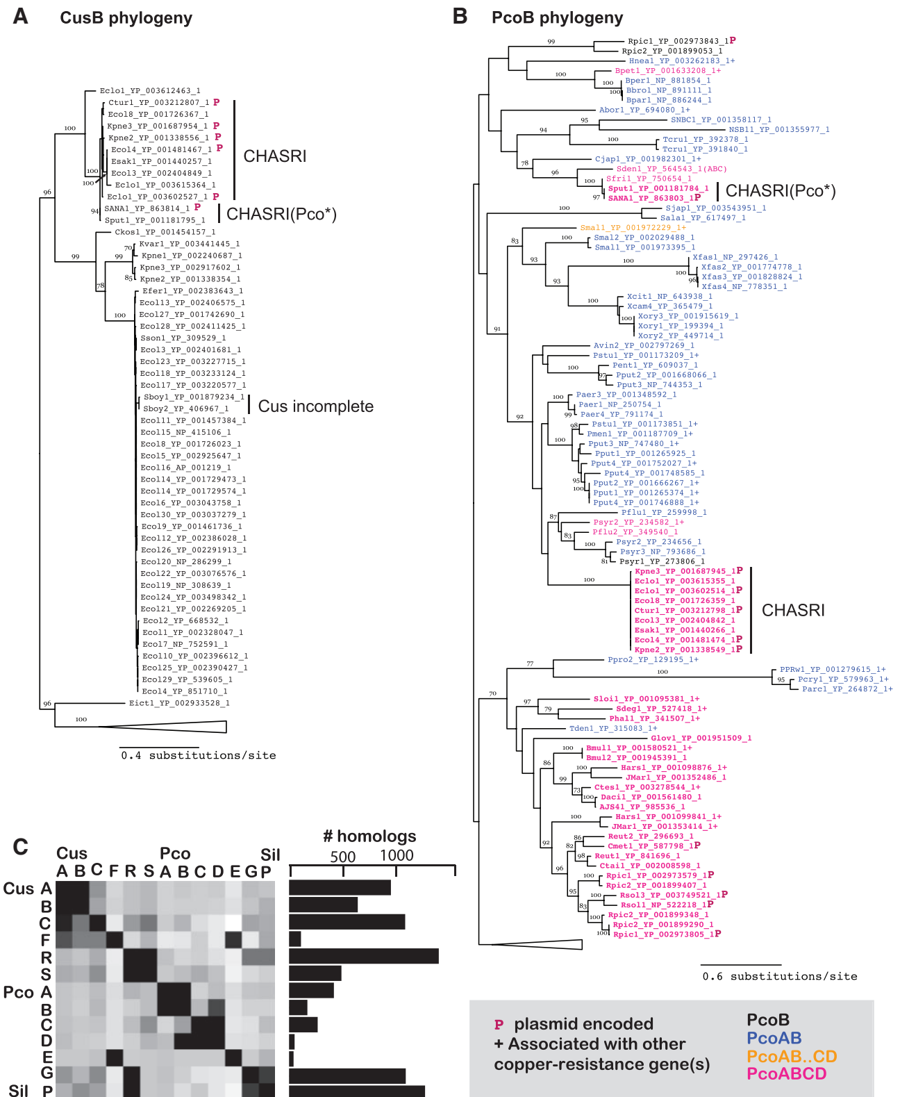
FIG. 5. —Diversity of CHASRI proteins. (A) ML amino acid phylogenies of CusB. (B) ML amino acid phylogenies of PcoB. Support values out of 100 ML bootstrap replicates are shown when \geq 70 . Color key displays clustering with functionally related genes. (C) The left panel is a heatmap of correlation of gene phylogenies expressed as the product of the proportion of shared reciprocal best BLAST hits for each gene, normalized by row. The right panel shows the number of homologs detected and analyzed for each gene.
