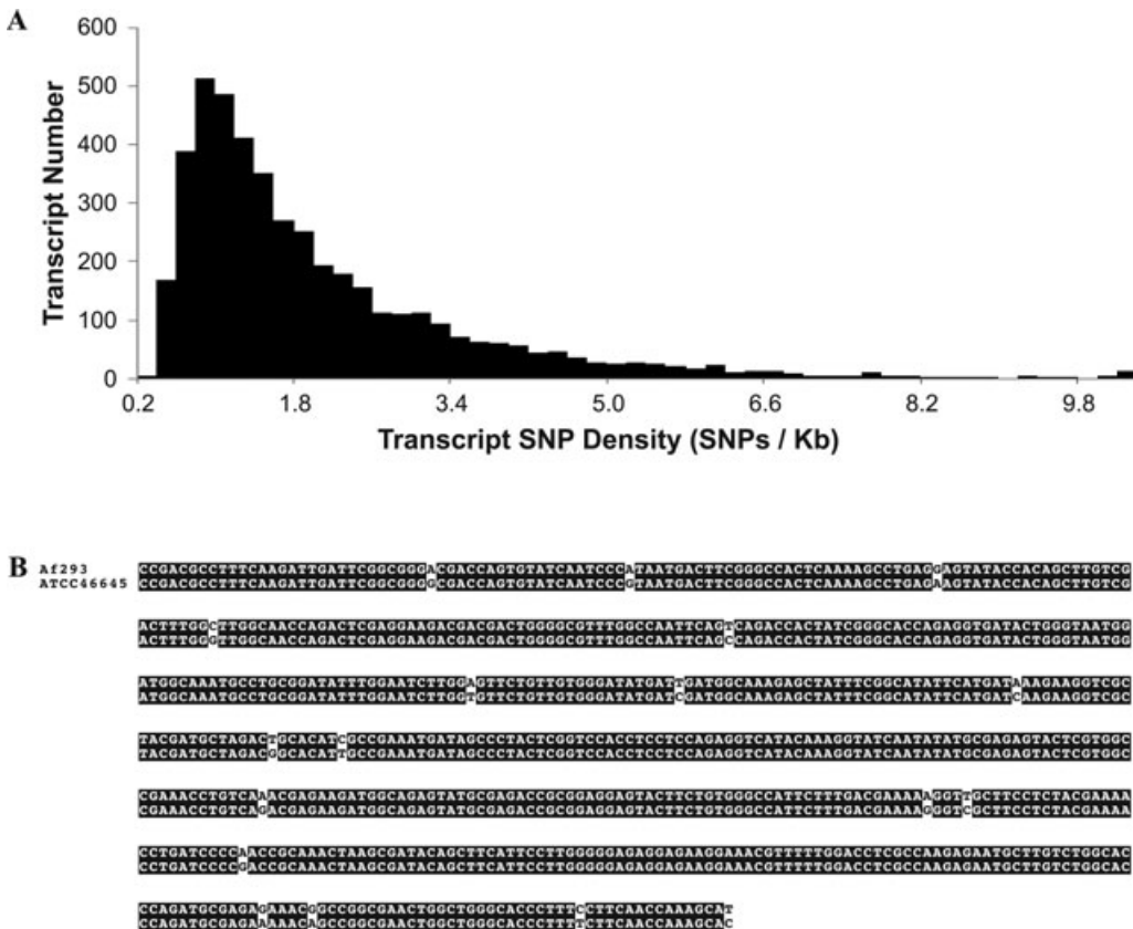
Figure 3. Transcriptome-wide variation between A. fumigatus strains ATCC46645 and Af293. (A) Histogram plot of transcript SNP density. The x-axis corresponds to groups of different transcript SNP densities (number of SNPs/Kb). The y-axis corresponds to the number of transcripts in each SNP density group. (B) Partial nucleotide sequence alignment between Af293 and ATCC46645 strains for a putative protein kinase (Afu3g03740), one of the genes with the highest SNP density in our comparison (see also Table 2). High-quality SNPs were identified by filtering for variable sites with coverage values \geq 5 and an average quality scores \geq 20 using the cns2np script in the Maq software. 35 Pairwise nucleotide diversity was calculated as \pi = n/N , where n is the number of differences between sequences, and N is the total number of sites examined. SNP density per Kb was calculated as \pi * 1,000 .
