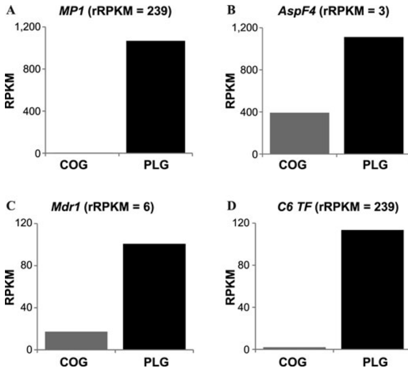
Figure 5. Examples of differentially regulated genes from specific functional categories that constitute candidates for the observed pathobiological and morphological differences between the two conditions. (A) The cell wall galactomannoprotein MPI (Afu4g03240). (B) The allergen AspF4 (Afu2g03830). (C) The ABC multidrug transporter Mdr1 (Afu5g06070). (D) The C6 transcription factor of the fumitremorgin secondary metabolism gene cluster (Afu8g00420). In each graph, the x-axis corresponds to the two growth conditions (COG in black and PLG in gray) and the y-axis to the RPKM expression value of the corresponding gene in each of the two conditions. The rRPKM (RPKM [COG]/RPKM [PLG]) value for each comparison is reported in parentheses next to each gene's name.
