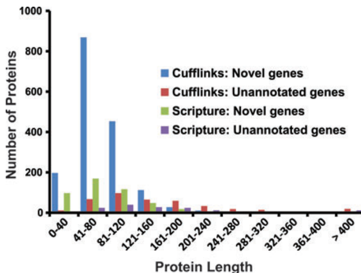
Figure 2. The majority of putative novel genes identified by RNA-seq in A. fumigatus encodes for small proteins. ATCC46645 sequence reads were mapped against the A. fumigatus Af293 reference genome with the TopHat software, 27 using the reference gene models 23 as guides and not allowing for introns >1,000 bp. Mapped reads were assembled into transcripts using the Cufflinks 25 and Scripture 26 programs, and their gene predictions were compared to the reference gene models. ORFs overlapping with exons of any reference gene model were classified as “annotated” genes. For the remaining ORFs, their protein products were searched against the NCBI nr database; these loci were classified either as “unannotated,” if the encoded protein had at least one homolog in the NCBI nr database, or as “novel,” if the encoded protein had no homologs in the NCBI nr database. The x-axis corresponds to groups of protein lengths encoded by putative novel or unannotated genes identified by the Cufflinks and Scripture programs (indicated by bars of different colors). The y-axis corresponds to the number of genes belonging to each group.
