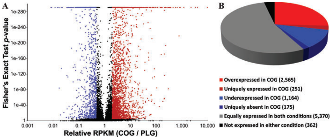
Figure 4. RNA-seq identifies thousands of differentially expressed genes from A. fumigatus ATCC46645 grown in the colony (COG) and plankton (PLG) growth conditions. (A) Volcano plot of the differentially regulated genes between COG and PLG conditions. For each gene, the rRPKM value (RPKM [COG]/RPKM [PLG]) was plotted against its respective Fisher's exact test P value. P values smaller than 1e^{-290} were reported as 1e^{-290} . The dotted line running parallel to the x -axis indicates the statistical cutoff ( P < 5.5e^{-6} ), whereas the dotted line running parallel to the y -axis indicates the biological cutoff (twofold difference in RPKM between COG and PLG). The red-colored and blue-colored dots correspond to upregulated and downregulated genes between COG and PLG, respectively. (B) Pie chart showing the partitioning of the 9,887 A. fumigatus genes with respect to their expression profile in the two growth conditions.
