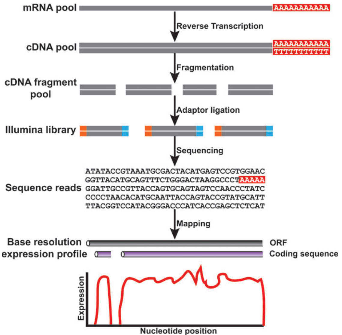
Figure 1. The workflow of a typical RNA-seq experiment. In brief, following isolation, the mRNA pool is converted to a cDNA pool and is then fragmented. Next, NGST adaptors are added to each cDNA fragment, the resulting library of fragments is sequenced, and the sequence of each fragment is read using NGST. Once sequence reads have been obtained, they can be used for a variety of analyses. For example, if the mRNA pool is from an organism whose genome and annotation is known, the sequence reads can be aligned or mapped to the reference genome or transcriptome and the sequence of the entire transcript as well as its relative expression can be calculated. Thus, RNA-seq technology is simultaneously qualitative (i.e., it can determine the sequences of different sequence fragments in a pool) and quantitative (i.e., it can determine the relative abundance of different sequence fragments in a pool).
